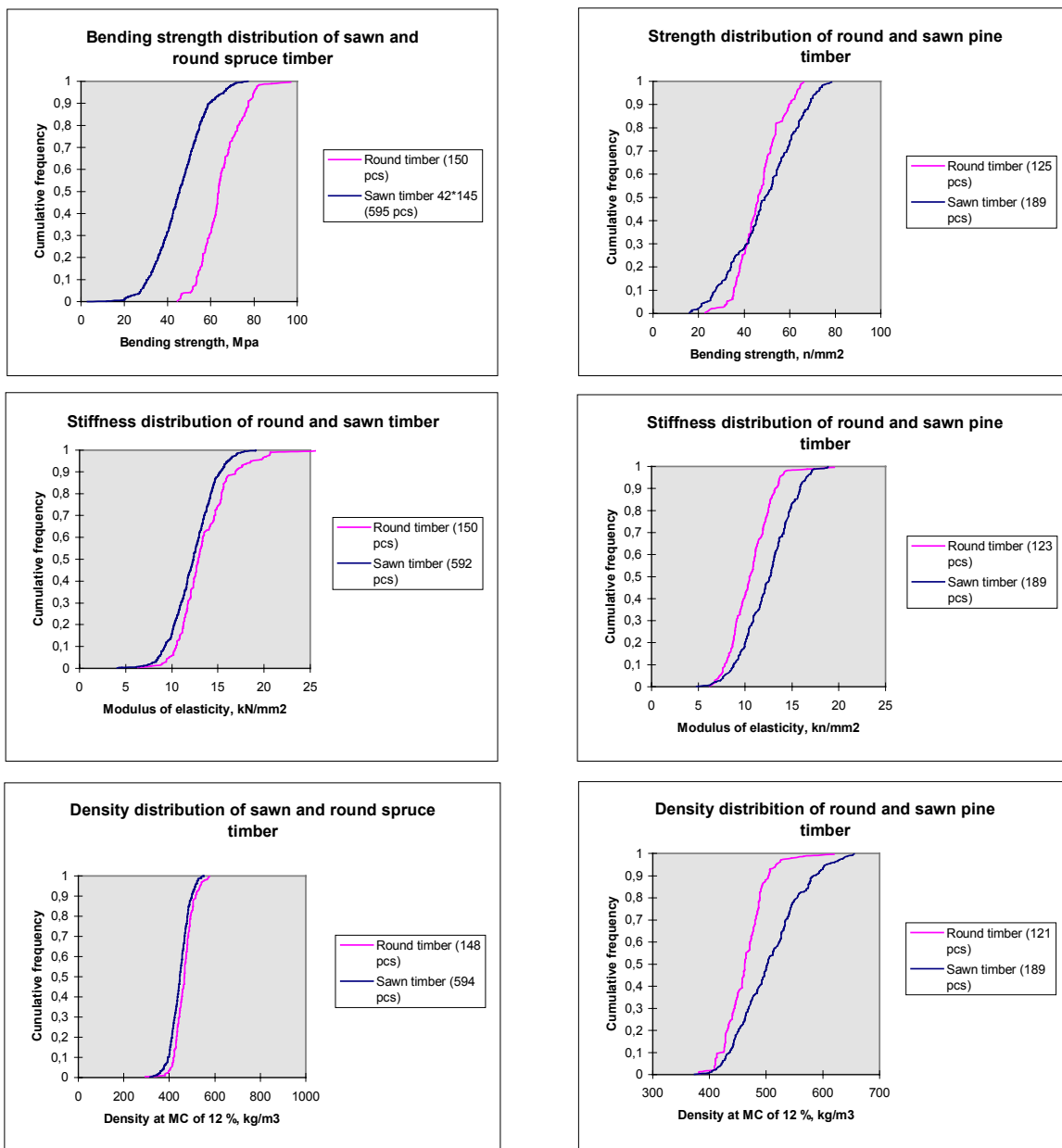
Figure 2. Comparison of bending strength, stiffness and density of round and sawn Finnish unsorted spruce and pine timber.
