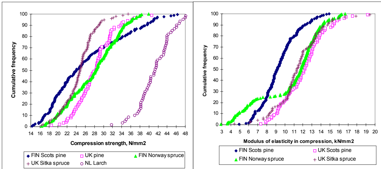
Figure 3. Cumulative frequencies of compression strength and modulus of elasticity by species at test moisture content.
